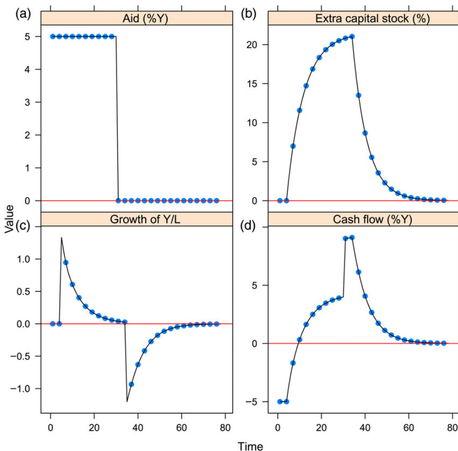
FIGURE 1. Paths of Selected Variables Under Baseline (physical capital) Simulation Threshold
