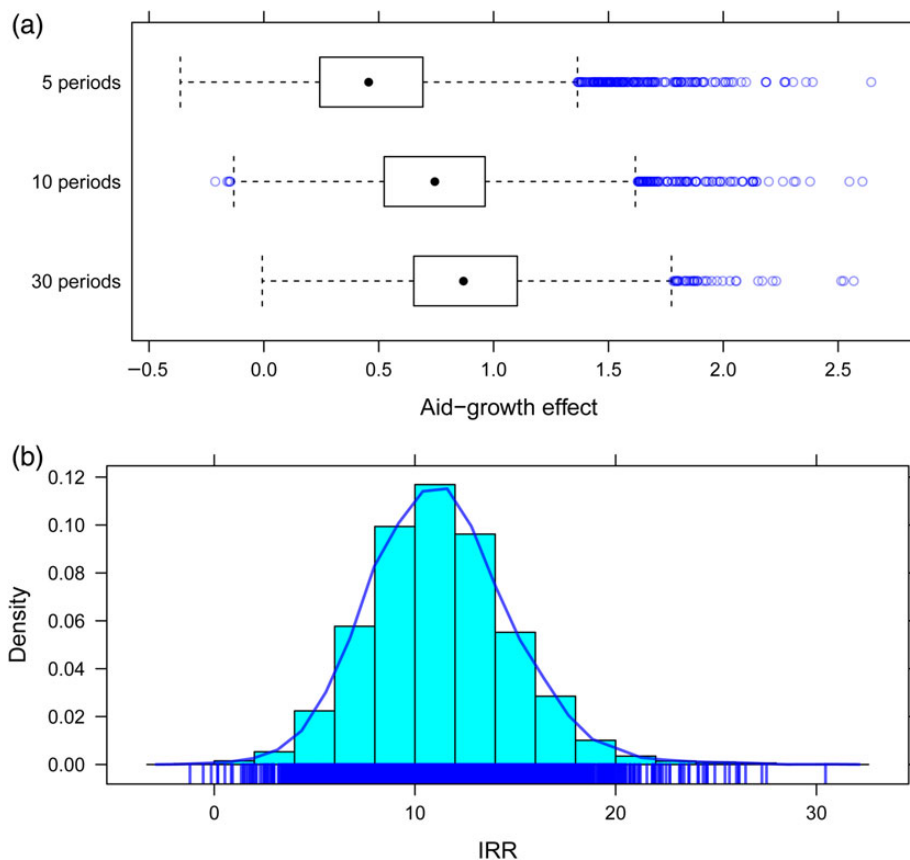
FIGURE 2. Summary of Aid-Growth and IRR Distributions, Full Model
